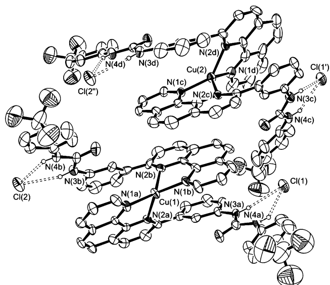
Figure 2. ORTEP view of the [\text{Cu}^{\text{I}}_2]\text{Cl} complex salt (names are only show for Cu, N, and Cl atoms; thermal ellipsoids are drawn at the 30% probability level; only hydrogen atoms bonded to the \text{N}_{\text{urea}} atoms are reported). The crystal contains two nonsymmetrically equivalent [\text{Cu}^{\text{I}}_2]^+ molecules and their counterions; each \text{Cl}^- ion interacts with four \text{NHCONH} (urea) groups as a proton acceptor of weak hydrogen bonds (drawn with dashed lines).
