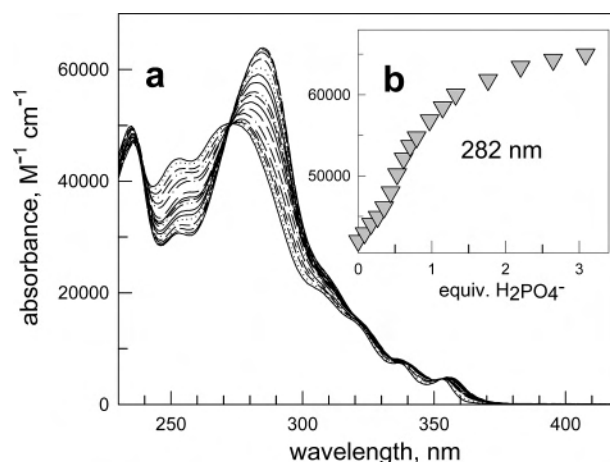
Figure 6. (a) Family of spectra obtained over the course of the titration of a solution 7.5 \times 10^{-6} M in 1 with a standard solution of [\text{Bu}_4\text{N}]\text{H}_2\text{PO}_4 in a 4:1 v/v THF:MeCN medium; (b) titration profile based on the absorbance at 282 nm.
