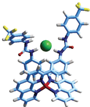
Figure 1. Hypothesized structure of the [\text{Cu}^{\text{I}}_2 \cdots \text{Cl}]^+ complex, which has been modeled through a semiempirical method (PM3).
