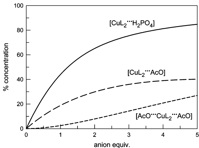
Figure 10. Medium: DMSO, 1 \times 10^{-4} M in [\text{Cu}^{\text{I}}(\mathbf{1})_2]^+ . Solid line: percent concentration of the [\text{Cu}^{\text{I}}(\mathbf{1})_2 \cdots \text{H}_2\text{PO}_4] complex over the course of the titration with \text{H}_2\text{PO}_4^- . Dashed lines: percent concentration of the [\text{Cu}^{\text{I}}(\mathbf{1})_2 \cdots \text{CH}_3\text{COO}] complex (long dashes) and the [\text{CH}_3\text{COO} \cdots \text{Cu}^{\text{I}}(\mathbf{1})_2 \cdots \text{CH}_3\text{COO}]^- complex (short dashes) over the course of the titration with \text{CH}_3\text{COO}^- . Percent concentration is given by the ratio of the current concentration of the receptor–anion complex [\text{Cu}^{\text{I}}(\mathbf{1})_2]^+ over the total concentration of the [\text{Cu}^{\text{I}}(\mathbf{1})_2]^+ receptor.
