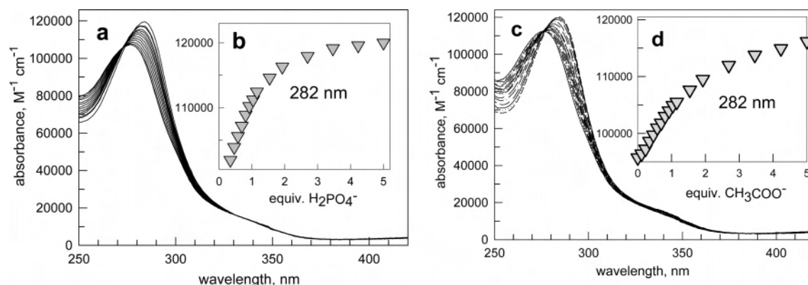
Figure 8. (a) Family of spectra obtained over the course of the titration of a solution 1.3 \times 10^{-4} M in [\text{Cu}^{\text{I}}(\text{I})_2]^+ with a standard solution of [\text{Bu}_4\text{N}]\text{H}_2\text{PO}_4 in a DMSO medium; (b) titration profile based on the absorbance at 282 nm; (c) family of spectra obtained over the course of the titration of a solution 1.3 \times 10^{-4} M in [\text{Cu}^{\text{I}}(\text{I})_2]^+ with a standard solution of [\text{Bu}_4\text{N}]\text{CH}_3\text{COO}^- ; (d) titration profile based on the absorbance at 282 nm.
