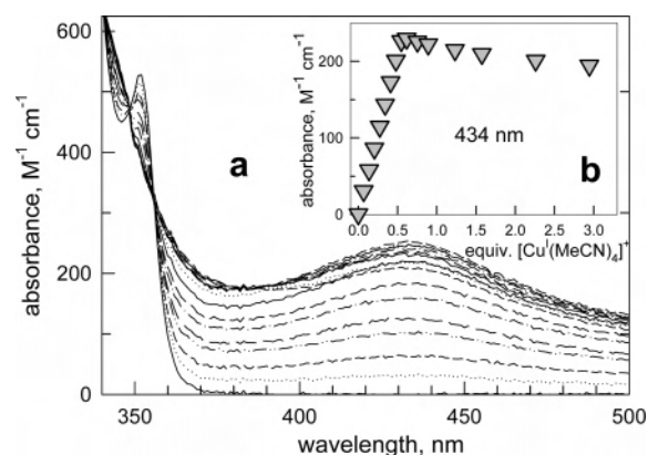
Figure 4. (a) Family of spectra obtained over the course of the titration of a solution 3 \times 10^{-4} M in 1 with a standard solution of [\text{Cu}^{\text{I}}(\text{CH}_3\text{CN})_4]\text{ClO}_4 in a 4:1 v/v THF:MeCN medium; (b) titration profile based on the absorbance of the band growing at 434 nm.
