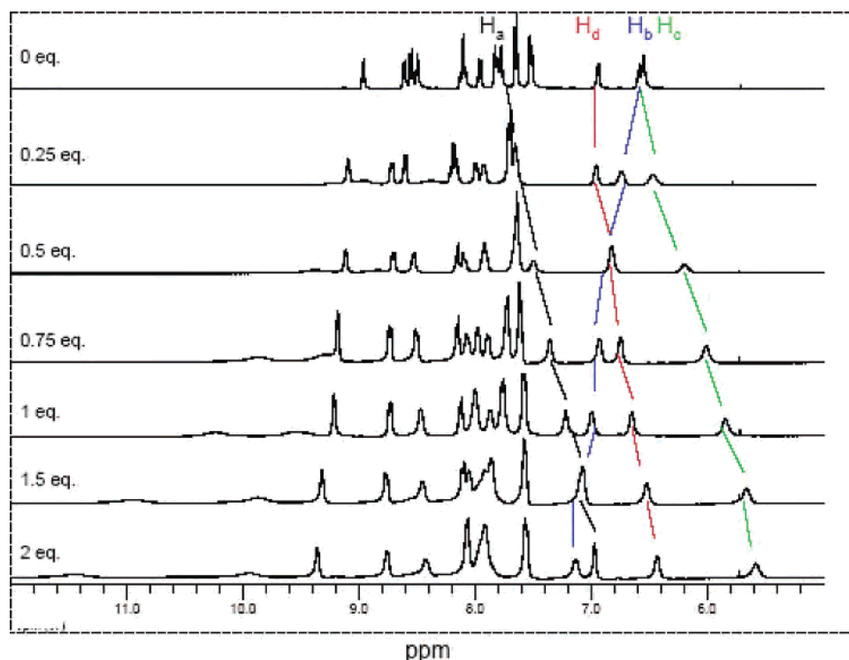
Figure 9. Family of spectra obtained over the course of the titration of a solution 6.0 \times 10^{-3} M in [\text{Cu}^{\text{I}}(\text{I})_2]^+ with [\text{Bu}_4\text{N}]\text{H}_2\text{PO}_4 in a 4:1 v/v DMSO- d_6 : \text{CD}_3\text{CN} medium.
