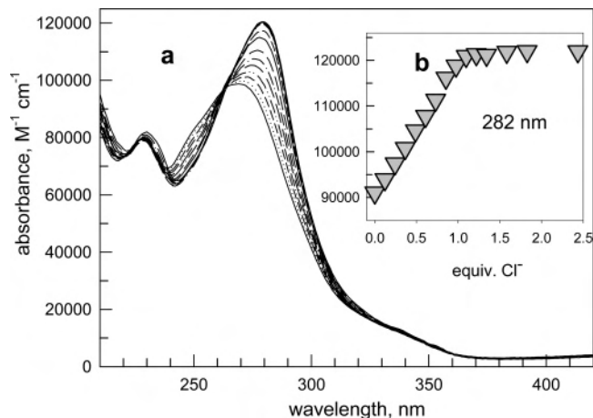
Figure 7. (a) Family of spectra obtained over the course of the titration of a solution 1.3 \times 10^{-4} M in [\text{Cu}^{\text{I}}(\mathbf{1})_2]^+ with a standard solution of [\text{Bu}_4\text{N}]\text{Cl} in a 4:1 v/v THF:MeCN medium; (b) titration profile based on the absorbance at 282 nm.
