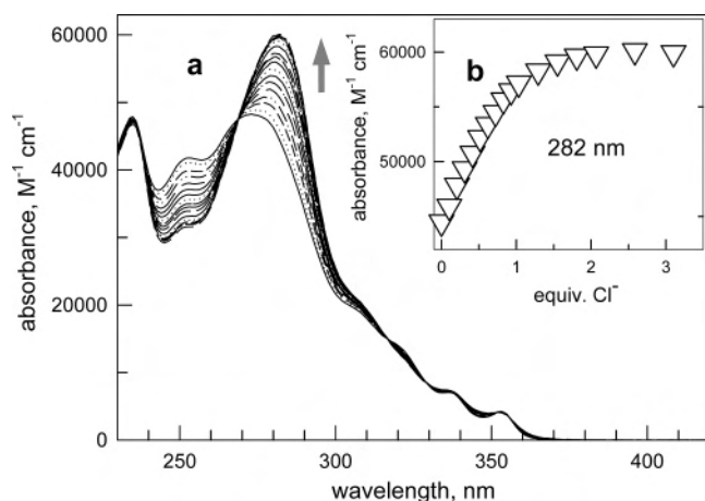
Figure 5. (a) Family of spectra obtained over the course of the titration of a solution 7.5 \times 10^{-6} M in 1 with a standard solution of [\text{Bu}_3\text{BzN}]\text{Cl} in a 4:1 v/v THF:MeCN medium; (b) titration profile based on the absorbance at 282 nm.
