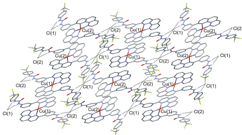
Figure 3. Simplified sketch of the molecular layer normal to the c axis; the extensive face-to-face \pi -stacking interactions between the aromatic groups of the [\text{Cu}^{\text{I}}(\mathbf{1})_2]^+ molecules are observed. Only H atoms bonded to the urea groups are shown, and the hydrogen-bond motifs involving NHCONH groups and \text{Cl}^- ions are drawn with dashed lines. Each of the chloride ions, Cl(1) and Cl(2), receives four hydrogen bonds.
